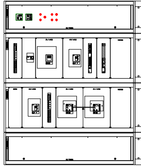
QUADRO POWER CENTER BT 20V GGBT TR2 E SCAMBIORETEGE
